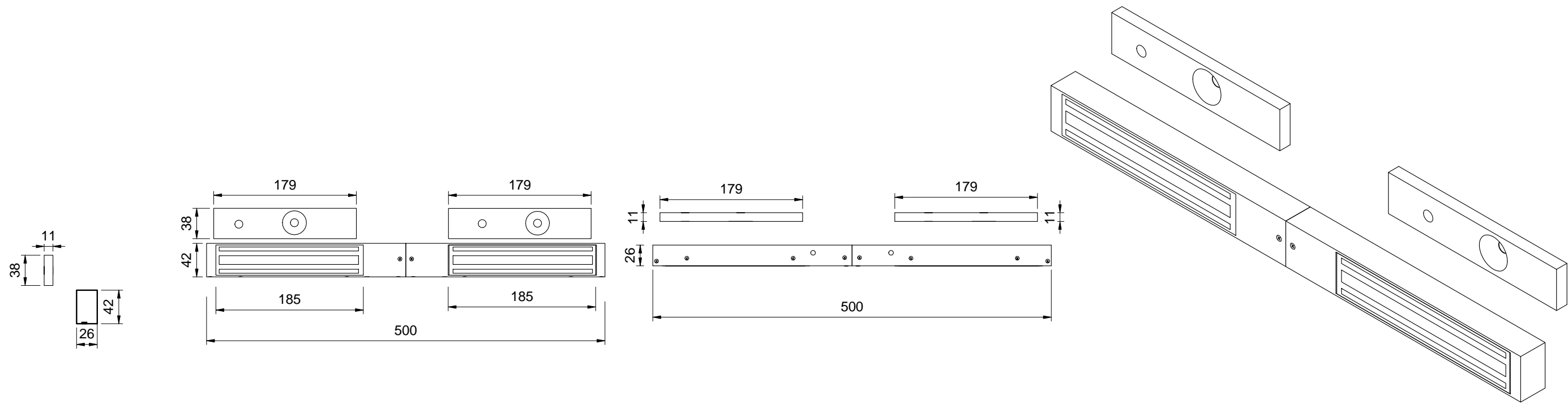
02 Side View 1 : 5
