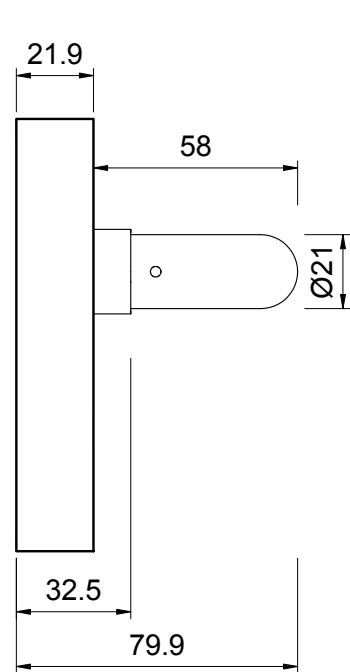
02 Side View 1 : 2
