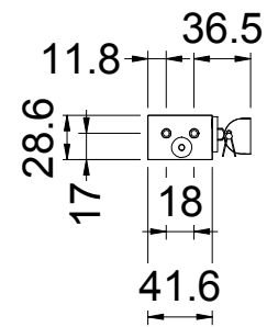
02 Side View 1 : 5
