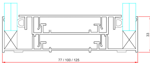
IQ Pro Floor & Ceiling Track
