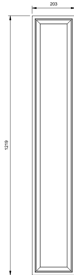
03 Front View 1 : 10
