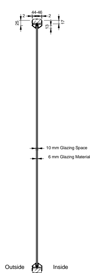
02 Side View 1 : 10
